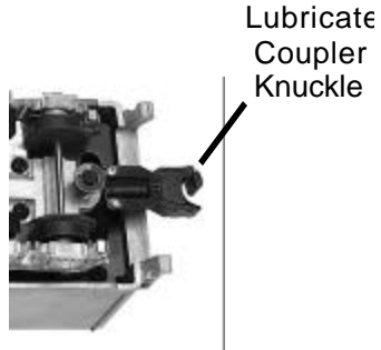
Figure 5: Lubricating The Coupler
