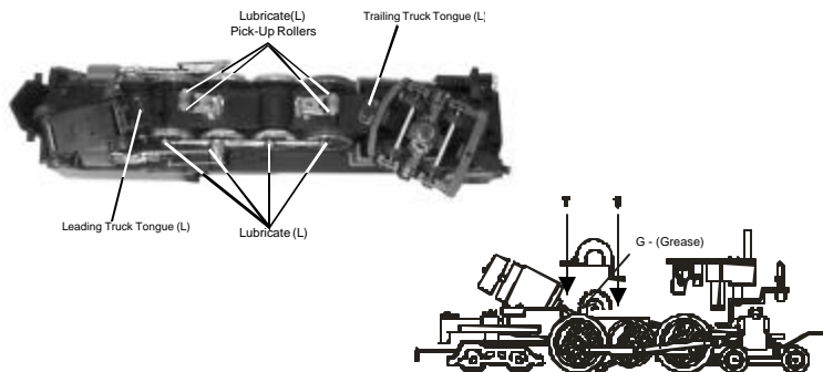
Figure 8: Lubricating The Locomotive Chassis
