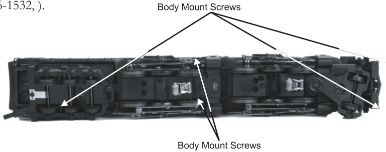
Figure 14: Remove Body Mount screws to get to the boiler
