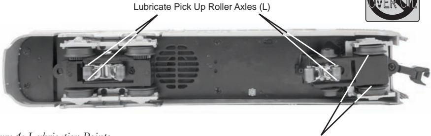
Figure 4: Lubrication Points
