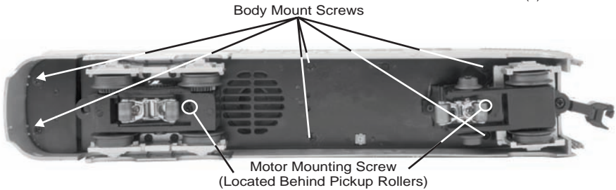
Figure 5: Body Removal Screw Locations and Motor Mounting Screws
