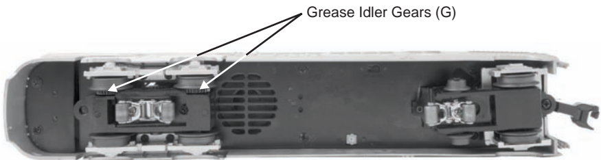
Figure 6: Greasing The Idler Gears
