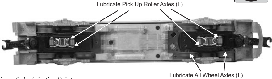
Figure 6: Lubrication Points
