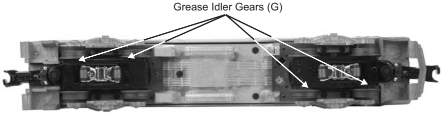
Figure 8: Grease Points
