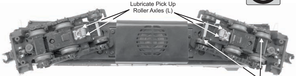
Figure 6: Lubrication Points
