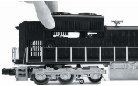
2. Remove Fan Cover to Access Smoke Unit and Volume Controls
