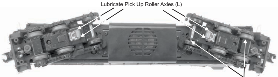
Figure 1: Lubrication Points on the Locomotive
