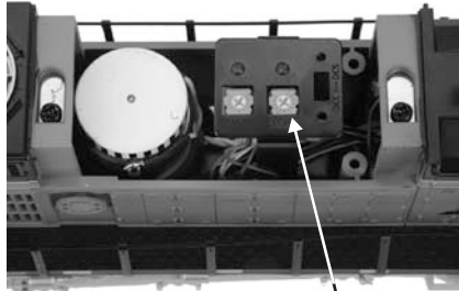
4. Smoke Unit Control Smoke Unit Control
