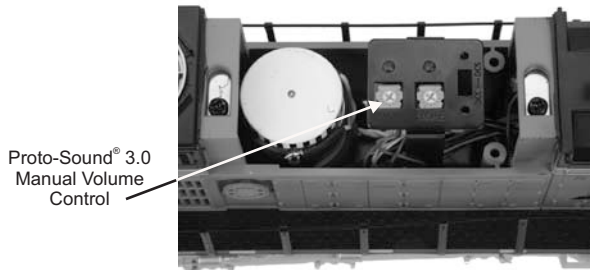
Figure 5: Manual Volume Control
