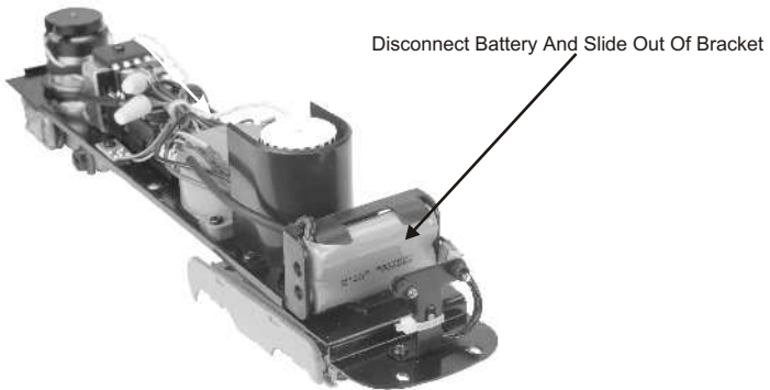
Figure 8. Battery Location.
