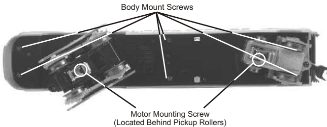
Figure 4. Body Removal Screw Locations
