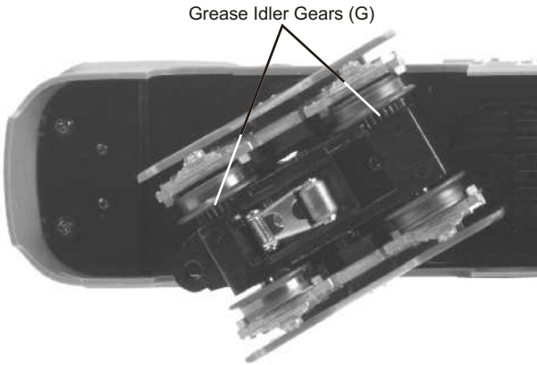
Figure 5. Greasing The Idler Gears
