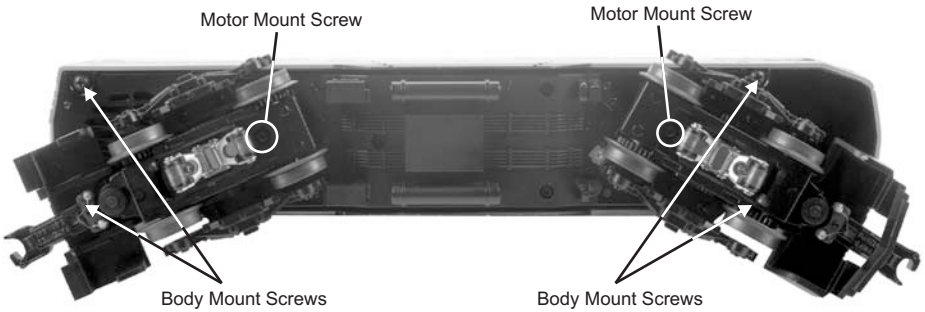
Figure: Body Removal Screw Locations and Motor Mounting Screws
