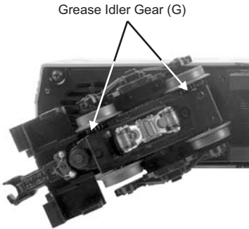
Figure: Greasing the Idler Gears
