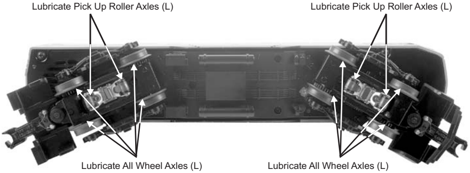
Figure: Lubrication Points on the Locomotive
