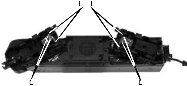
Figure 6: Lubricating The Locomotive Chassis
