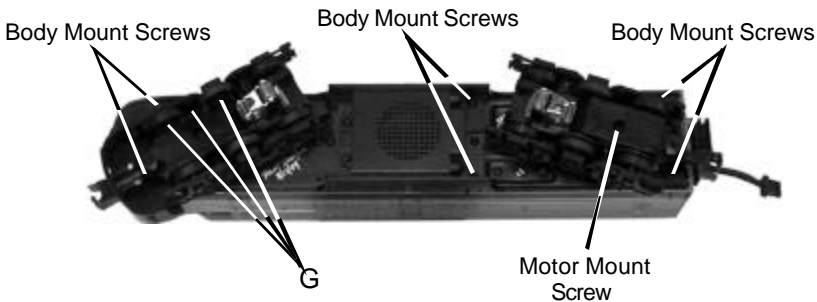
Figure 7: Lubricate The Tender Chassis Trucks
