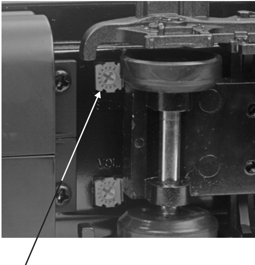
Figure 3: Smoke Unit Control
