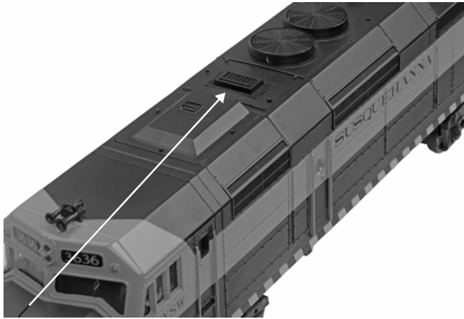
Figure 2: Adding Smoke Fluid
