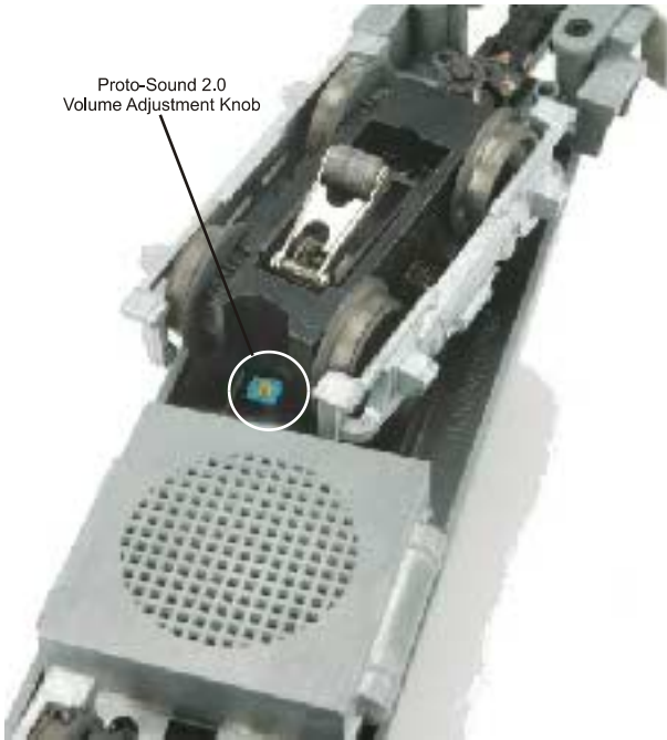
Figure 2. Manual Volume Adjustment Knob
