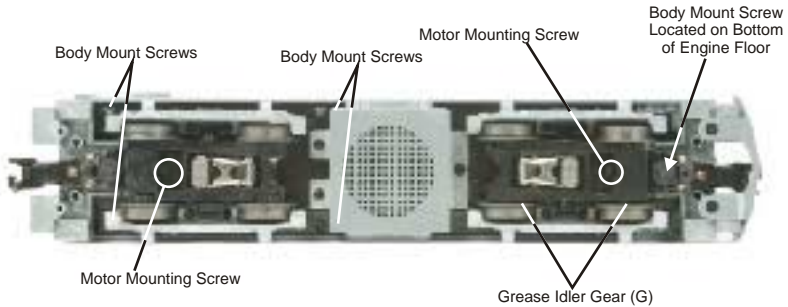
Figure 3. Body Removal Screw Locations
