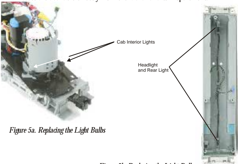
Figure 5b. Replacing the Light Bulbs
