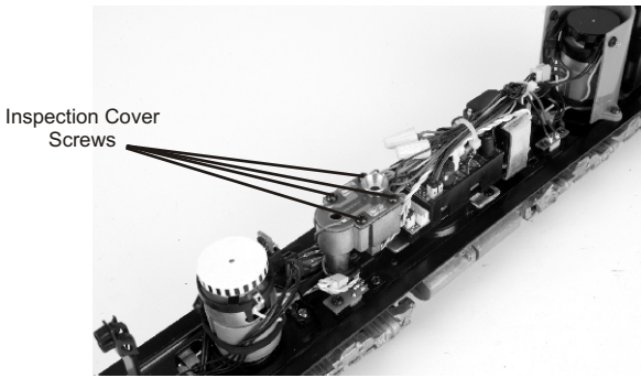
Figure 8. Inspecting the Smoke Unit Wick
