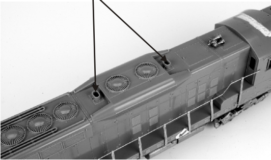
Figure 2. Adding Smoke Fluid
