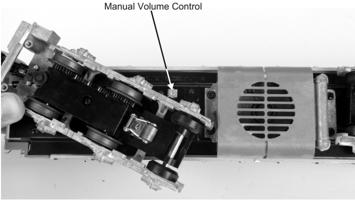
Figure 4. Manual Volume Control
