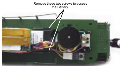
Figure 6. Removing and Replacing the Battery
