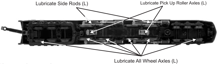
Fig. 9: Lubricating the Locomotive
