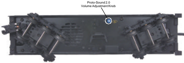
Figure 4: Manually Adjusting The Volume
