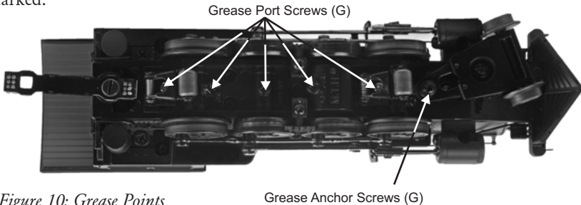
Figure 10: Grease Points
