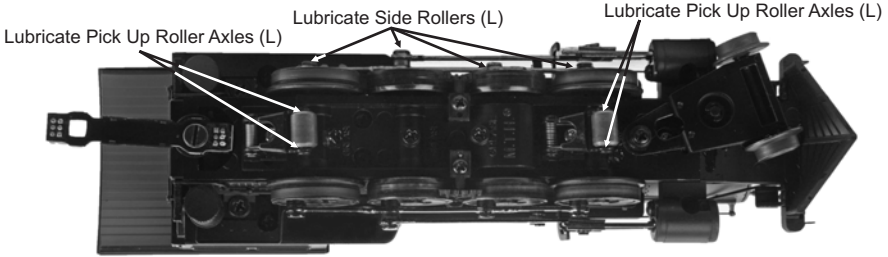
Figure 9: Lubricating the Locomotive Lubricate All Wheel Axles (L)
