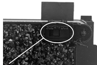
Figure 7: Changing from DCS to DCC Mode
