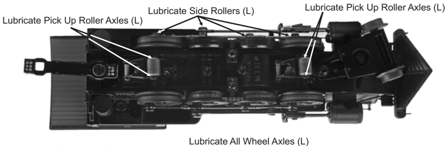
Fig. 1: Lubricating the Locomotive
