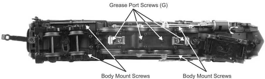
Figure: Grease Points & Body Mount Screw Locations
