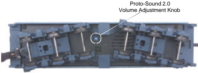
Figure 4: Manual Volume Adjustment
