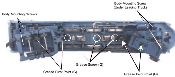
Figure 6: Removing The Body
