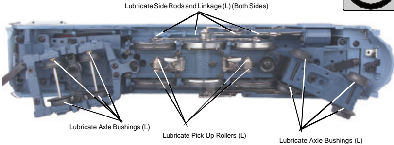
Figure 5: Lubricating The Chassis
