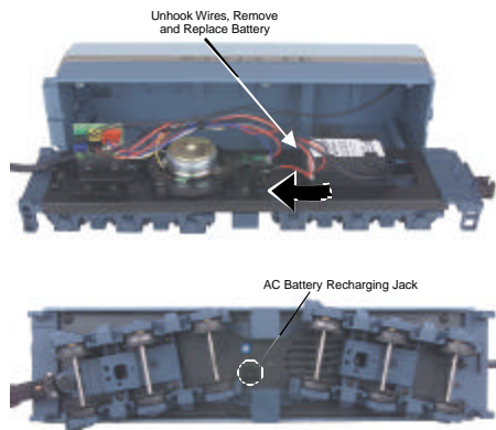
Figure 9: Replacing The Battery And Locating The Battery Recharging Jack
