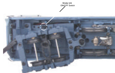
Figure 2: Smoke Unit Switch Location
