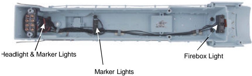
Figure 7: Headlight Wire Harness
