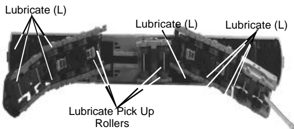
Figure 7: Lubricating The Trucks (Both Ends)
