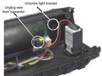
Figure 9. Changing the Tender Light.
