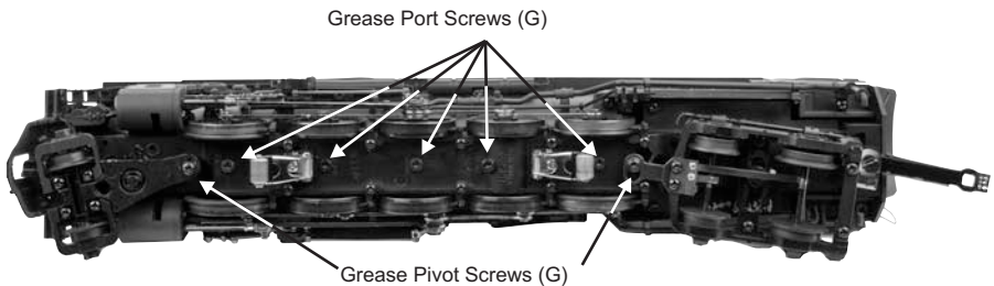
Figure 11: Grease Points
