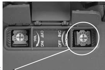
Figure 4: Smoke Unit Control
