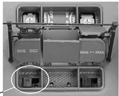
Figure 8: Changing from DCS to DCC Mode
