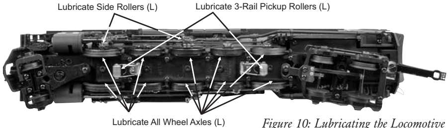
Figure 10: Lubricating the Locomotive
