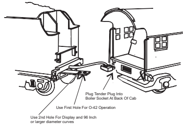
Figure 1: Pluggin in the tender harness
