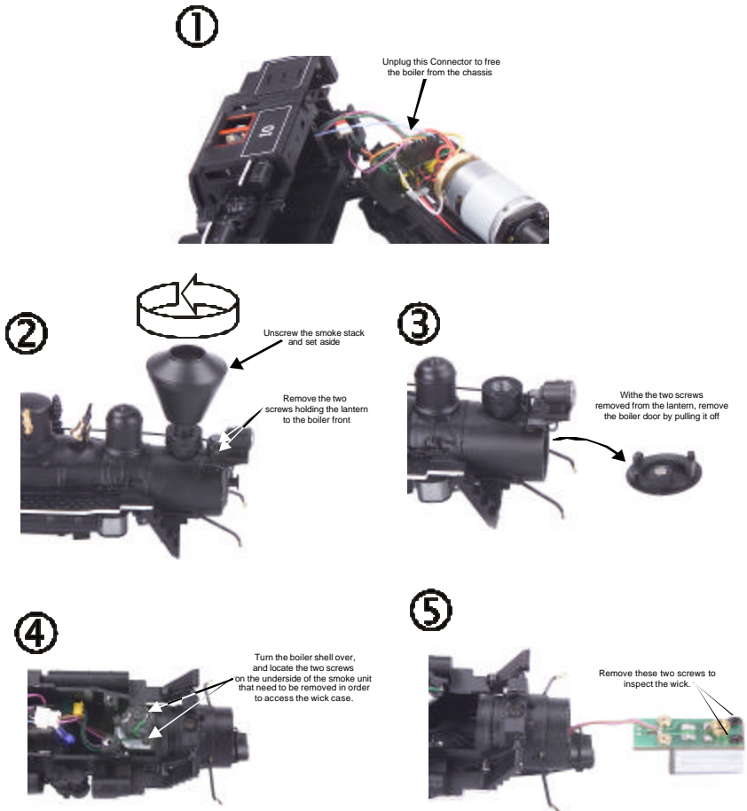
Figure 7. Accessing the Smoke Unit in the Boiler Shell
