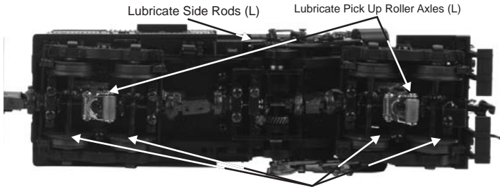
Fig. 1: Lubricating the Locomotive
