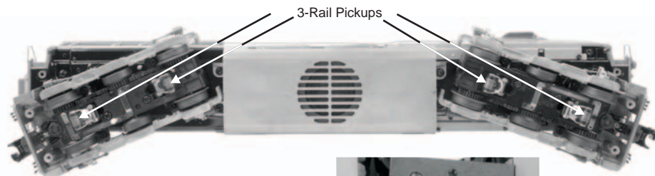
Figure 4: 3-Rail Pickups
