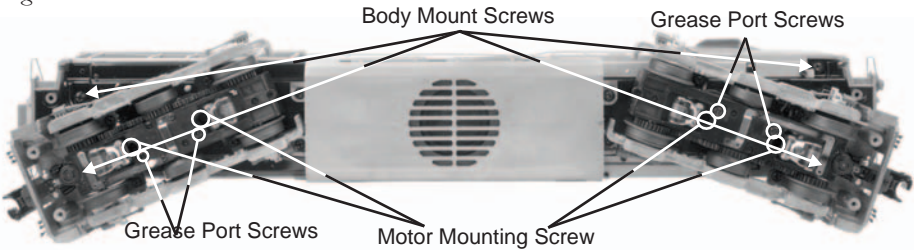
Figure 8: Lubrication Points
