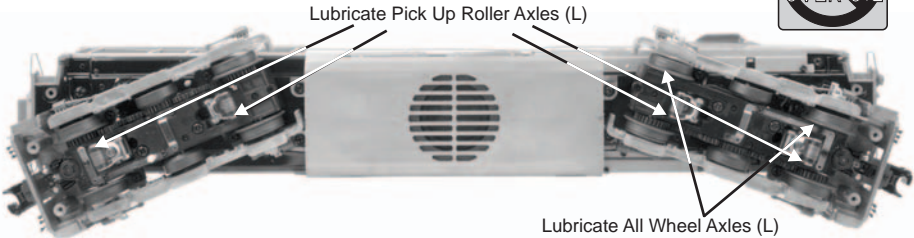
Figure 8: Lubrication Points
