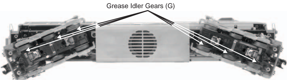
Figure 10: Greasing The Idler Gears
