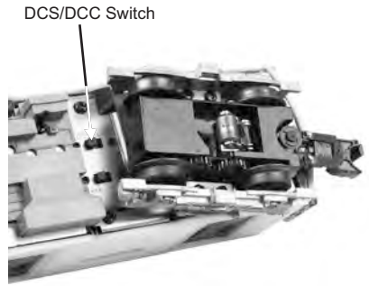
Figure: Changing from DCS to DCC Mode
