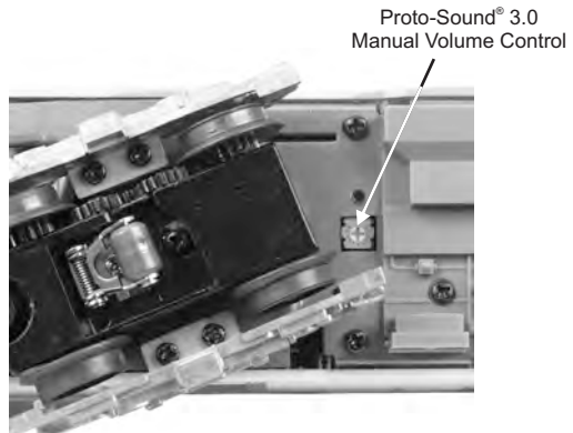
Figure: Manual Volume Control
