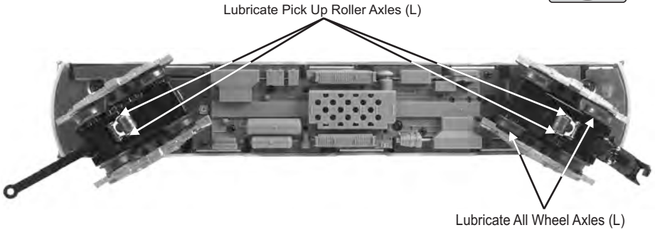
Figure: Lubrication Points
