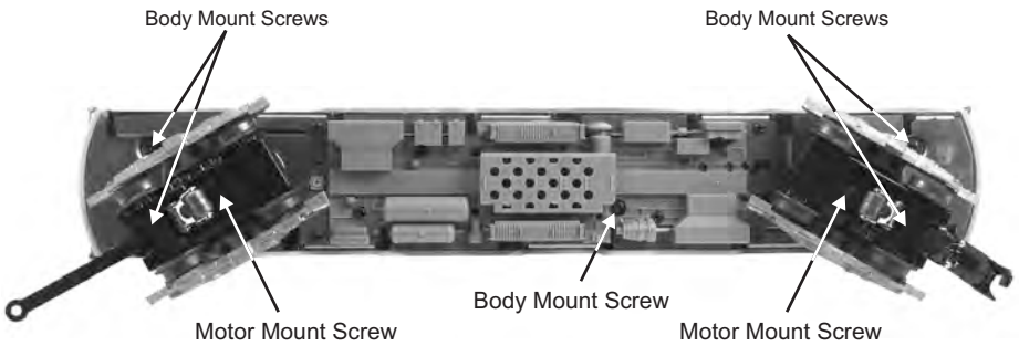
Figure: Body Mount and Motor Mount Screws
