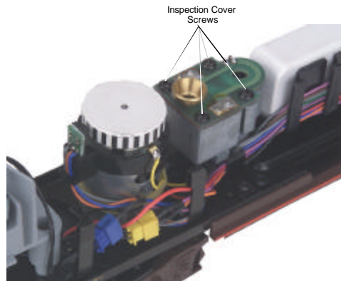
Figure 13: Inspecting The Smoke Unit Wick
