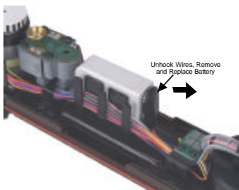
Figure 11: Removing the battery
