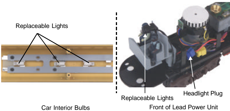
Figure 9: Replaceable light bulb locations
