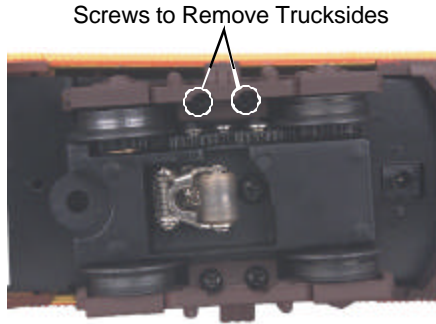
Figure 8: Removing the trucksides
