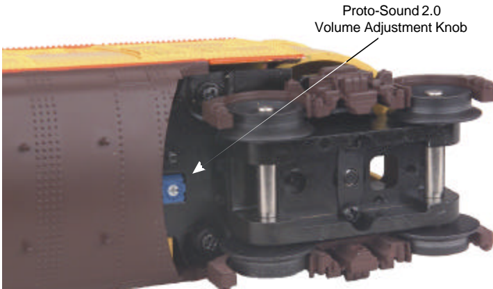
Figure 5: Proto-Sound Manual Volume Adjustment
