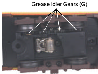
Figure 7 : Greasing the gears
