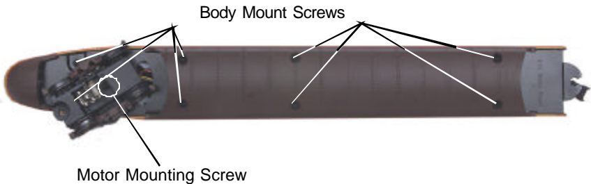
Figure 7: Removing the body from the observation car
