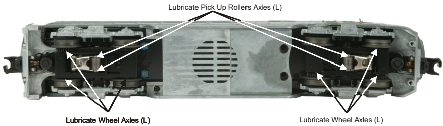
Figure 5. Lubrication Points on the Locomotive.
