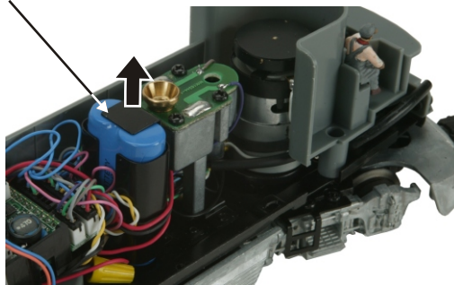
Disconnect Battery And Slide Out Of Bracket
