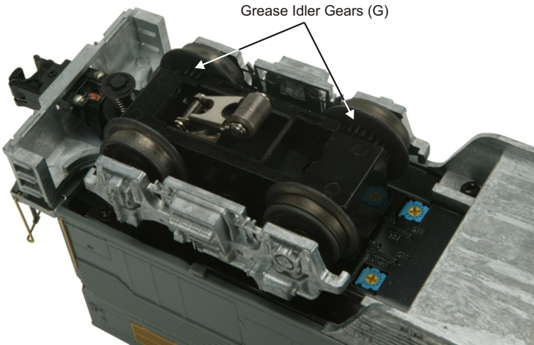
Figure 7. Greasing The Idler Gears
