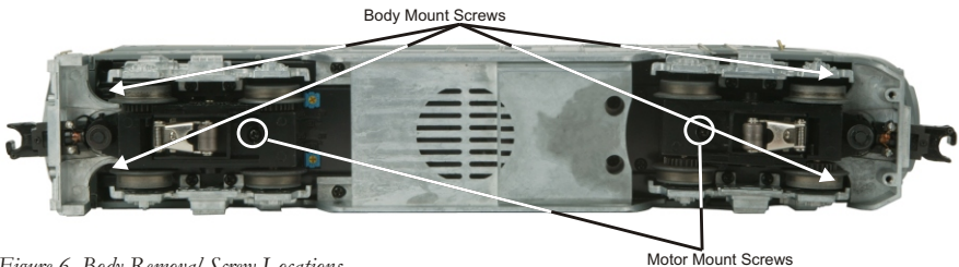
Figure 6. Body Removal Screw Locations
