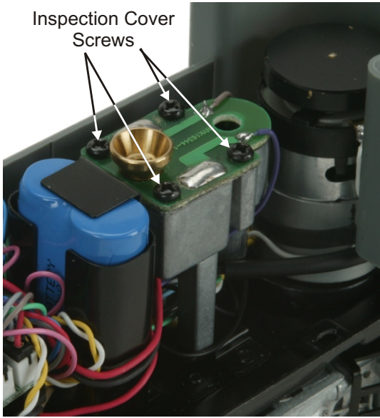
Figure 11. Inspecting the Smoke Unit Wick
