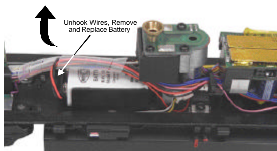
Figure 10: Removing The Battery
