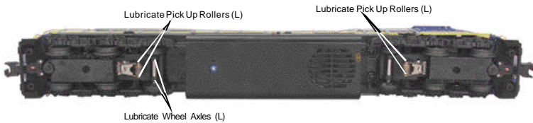
Figure 1. Lubrication Points on the Locomotive
