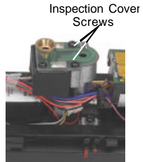
Figure 12 : Smoke Unit Inspection
