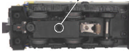
Figure 7: Removing The Truck Block To Access Trucksides Screws
