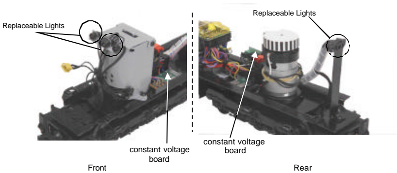
Figure 8: Removing The Replaceable Lights
