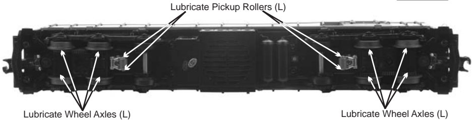
Figure 6. Lubrication Points on the Locomotive
