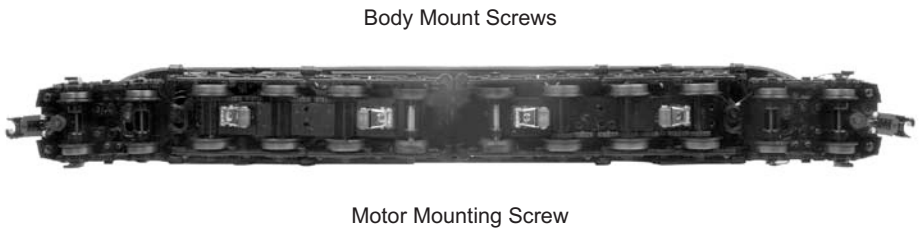
Figure 7. Body Removal Screw Locations and Motor Mounting Screws
