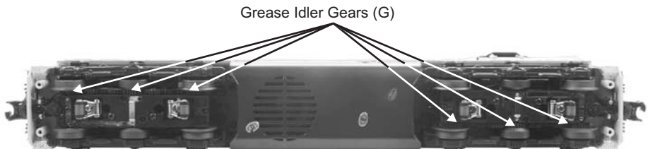
Figure 10: Greasing The Idler Gears
