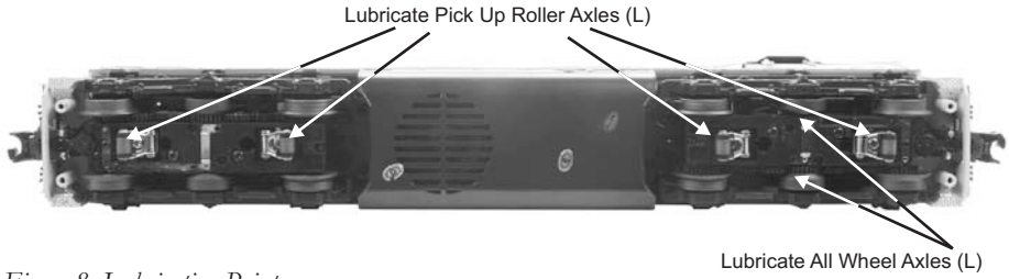
Figure 8: Lubrication Points
