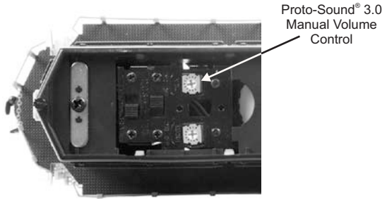
Figure 7: Manual Volume Control
