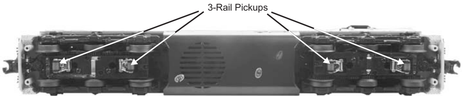
Figure 4: 3-Rail Pickups
