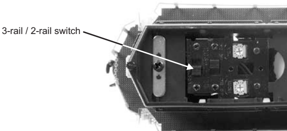
Figure 5: 3-Rail Pickups
