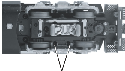
Truckside Screws
