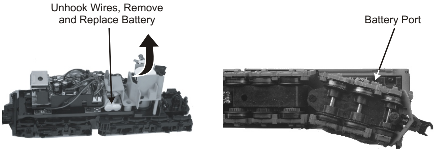
Figure 7. Replacing the Battery
