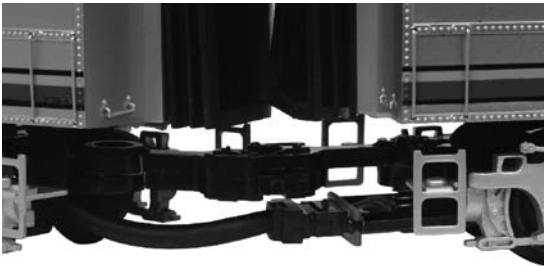
Figure 6: Correct way to Connect wire harness plug into the receptacle [The top of the plug will have the word 'TOP' imprinted on it]
