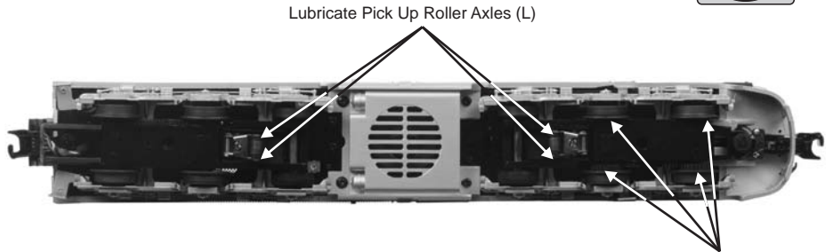
Figure 10: Lubrication Points on the Locomotive
