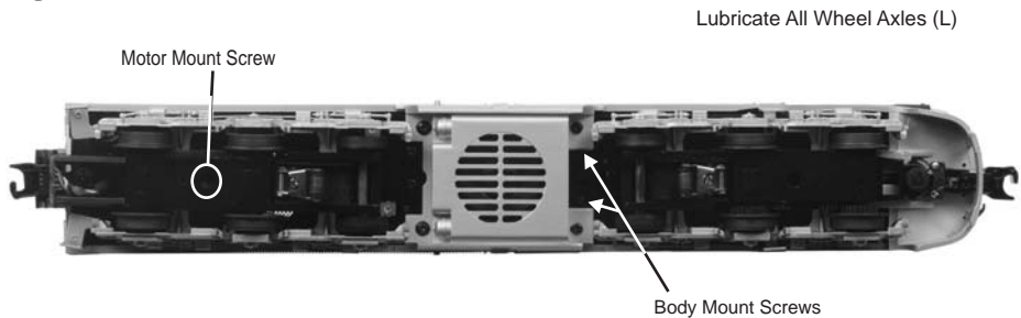
Figure 11: Body Mount Screws
