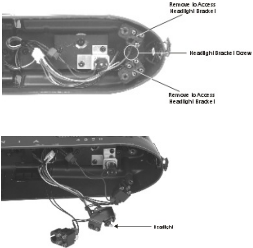
Figure 8. Removing the Headlight
