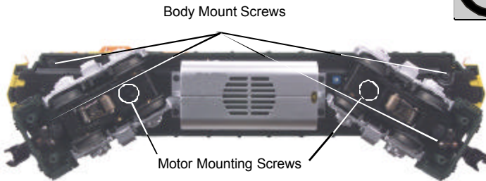
Figure 3: Body Removal Screw Locations
