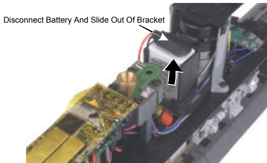
Figure 6: Removing The Battery
