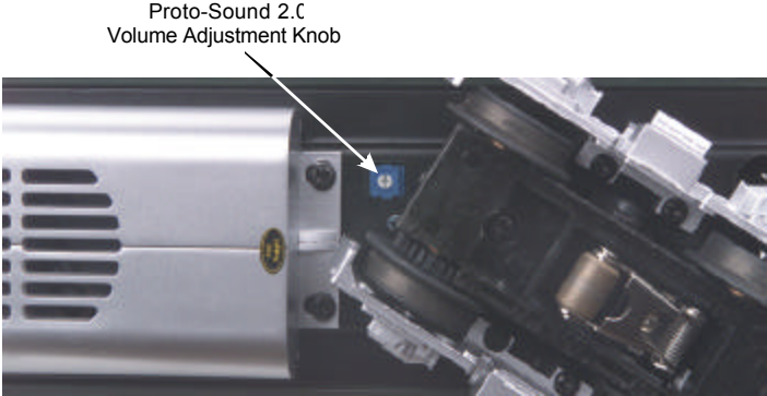
Figure 2: Manual Volume Adjustment Knob
