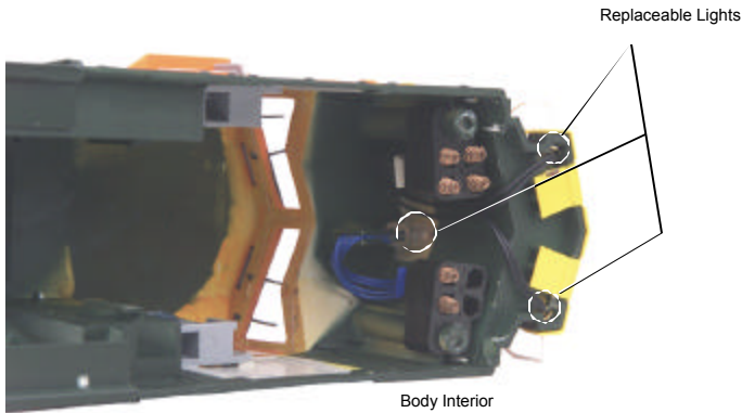
Figure 4: Removing The Replaceable Lights
