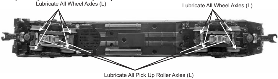
Figure 8: Lubrication Points on the Locomotive
