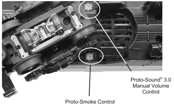
Figure 7: Manual Volume Control/Smoke Volume Control
