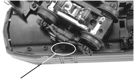
Figure 4: 2Rail/3Rail Switch & Smoke Control
