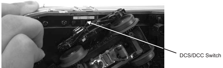
Figure 6: Changing from DCS to DCC Mode
