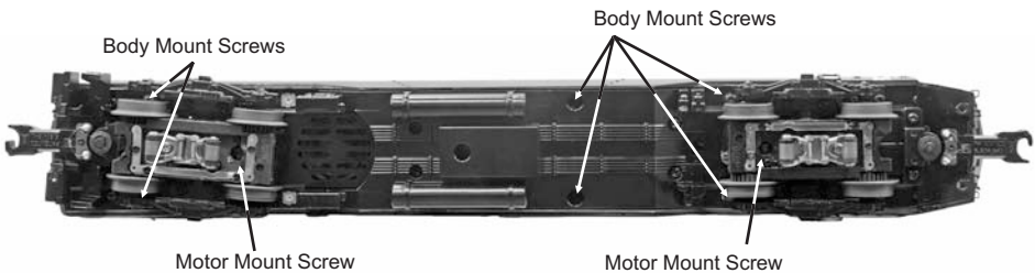
Figure 9: Body Mount Screws
