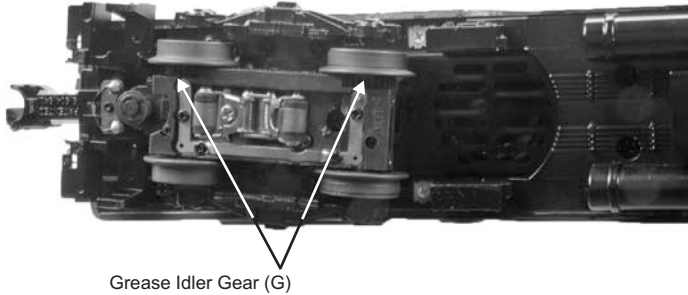
Figure 10: Greasing the Idler Gears
