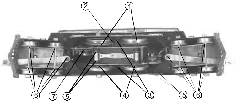
Figure 2: Lubricating Engine
